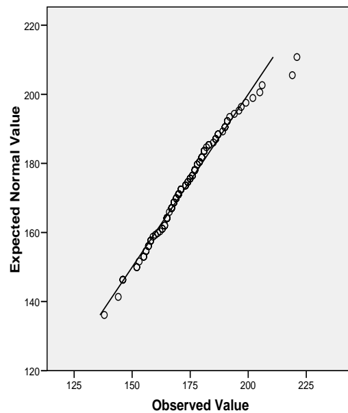
Normal Q-Q Plot of kecerdasan_emosional
